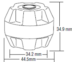
1603 SERIES 600 VOLT HIGH STRENGTH STANDOFF INSULATOR
