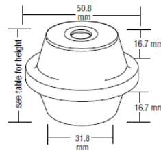
SERIES 2017 CENTER-POST INSULATORS
