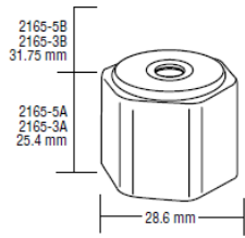
SERIES 2165 PANEL & SWITCHBOARD INSULATORS
